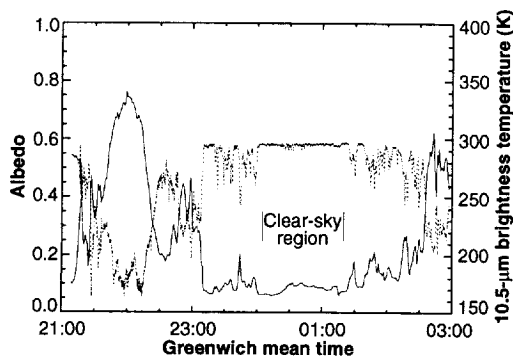
Fig. 2. RAMS 10.5-μm (nadir viewing) brightness temperature (dashed line) and broadband solar albedo (solid line) measured from the ER-2 during the flight on 15 March 1993 over the 2°S latitude belt between 180°E and 170°W. An example of data classified as clear sky is indicated.
