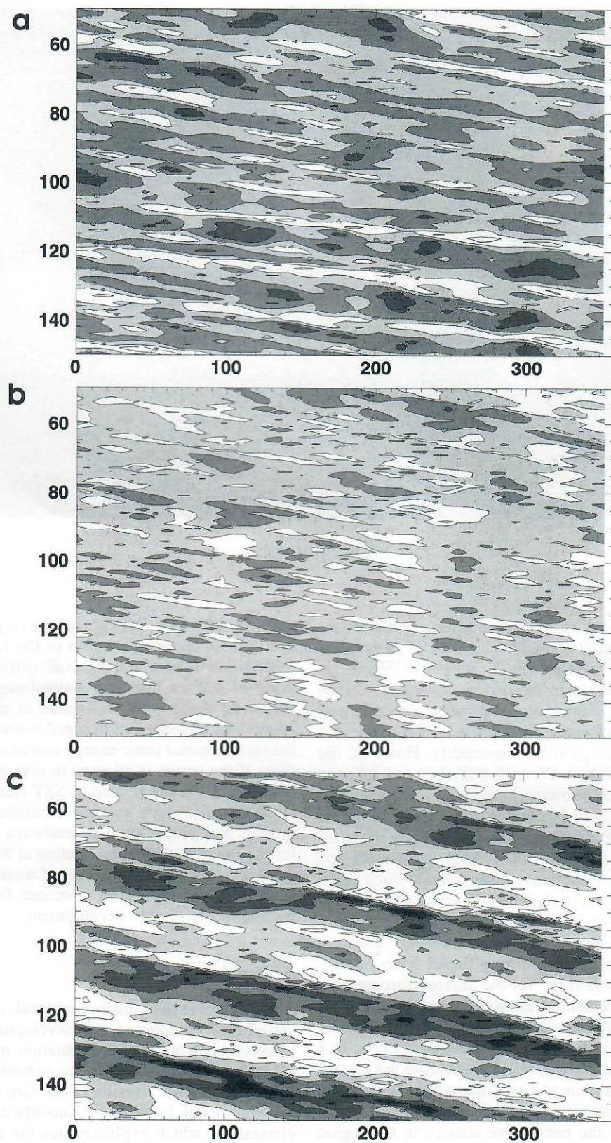
FIG. 10. Longitude-time (in days) diagram of the equatorial winds for (a) constant SST, (b) constant SST and wind-evaporation feedback removed, and (c) equatorial SST modified.
