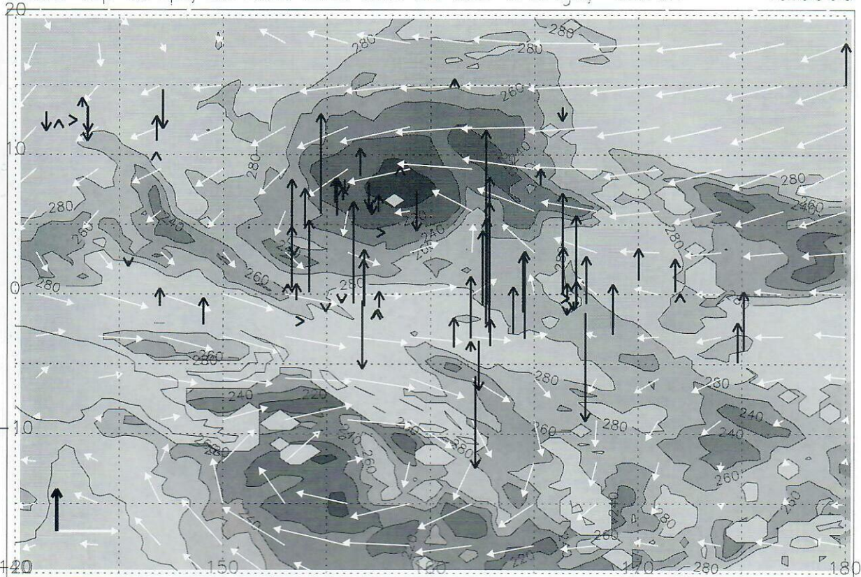
FIG. 2. NOGAPS surface (10 m) winds (white arrows), GMS cloud-top temperatures (shaded, in K), and drifters 24-h SST change (black arrows) on 13 March 1993. The scale in lower-left corner shows wind speed of 10 \text{ m s}^{-1} and 0.1^\circ \text{ day}^{-1} SST change.
