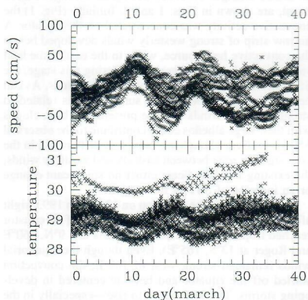
FIG. 3. Surface (15 m) currents and SST measured by Lagrangian drifters during March 1993. The buoys locations are between 3^\circ\text{S} and the date line.
