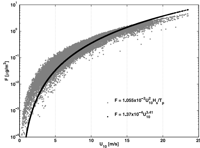
Figure 1. Sea salt mass emission as a function of surface wind velocity. Black points represent the reference (Monahan's) parameterization whereas gray points represent the proposed parameterization.
