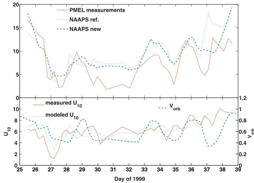
Figure 2. (top) Sea salt surface mass concentrations during Aerosols99 (Leg 1, Southern Hemisphere only) experiment. Solid line represents PMEL group observations; NAAPS results from two simulations, one with reference emission parameterization and the other with the proposed emission scheme are represented by dotted and dashed lines, respectively. (bottom) Left axis, ship measurements (solid line) and NOGAPS (dotted line) surface wind velocities; right axis, wave's orbital velocity (dashed line) ( V_{orb} = \pi H_s/T_p ).
