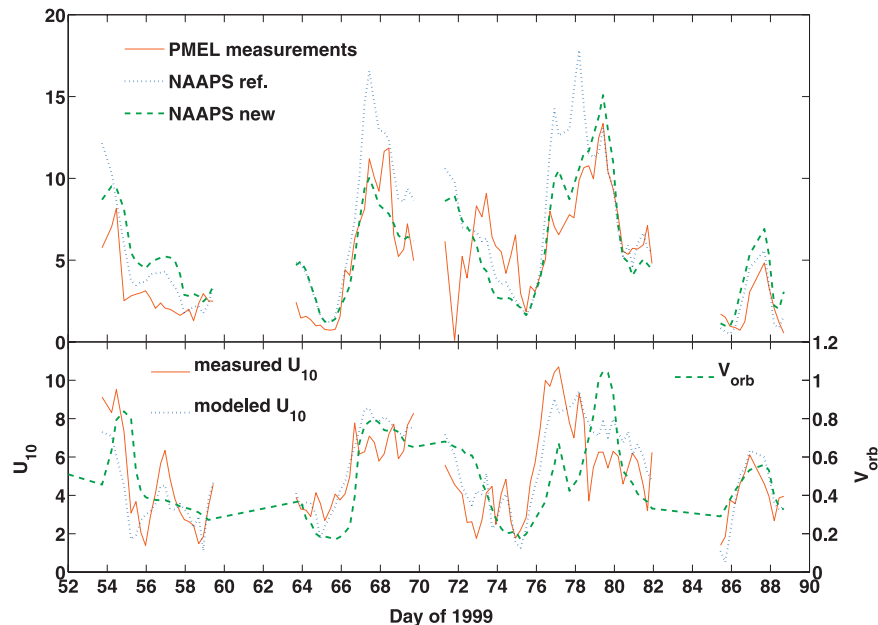
Figure 3. Same as Figure 2 but for INDOEX experiment.
